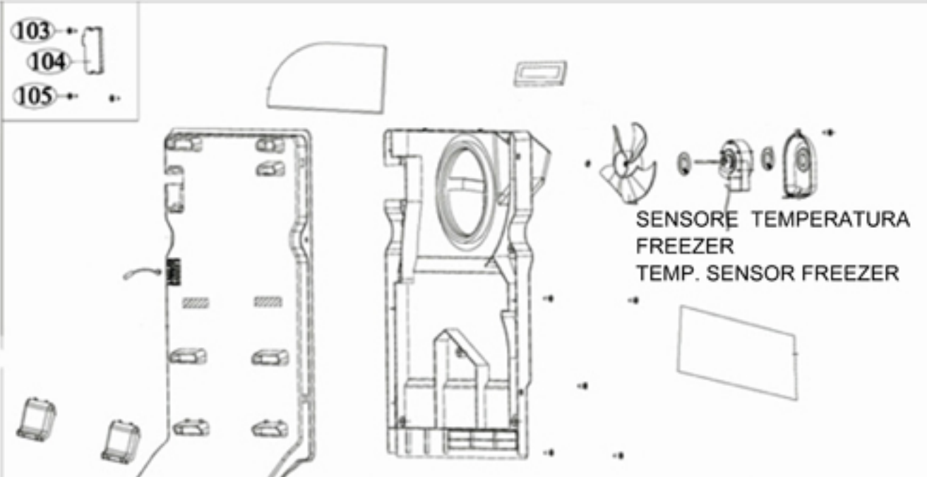
121 Freezer airflow assembly ASSIEME AIRFLOW CONGELATORE
